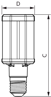
TrueForce LED HPL ND 6klm E40 840 CL IP65
